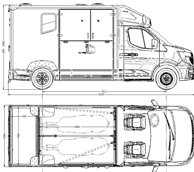
CABINE 3 PLACES
